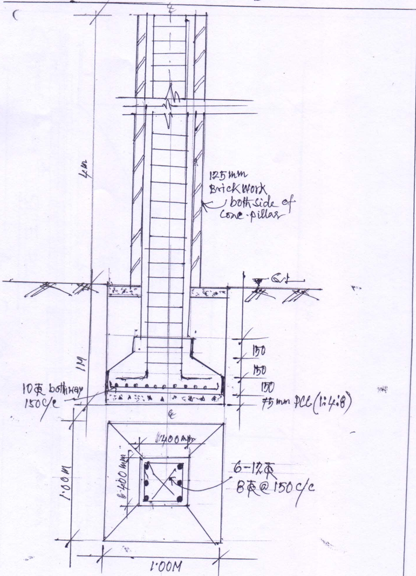
COLUMN FOUNDATION
